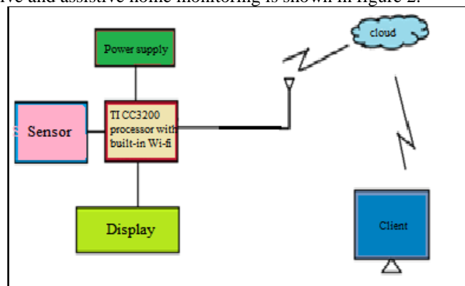
Figure 3: Implemented block diagram Proposed System for active-assisted living
