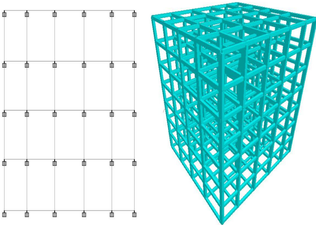
Fig1: Modeling in STAAD pro
