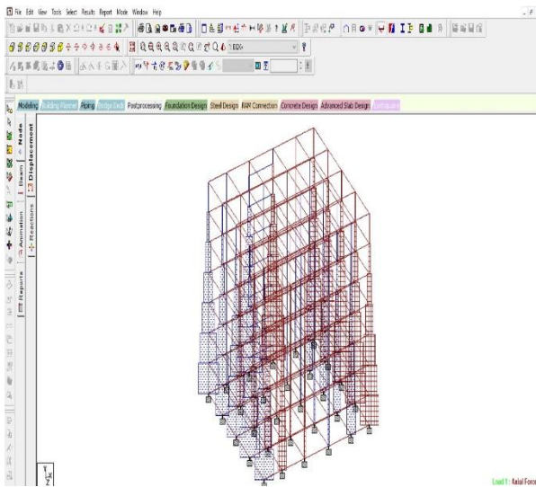
Fig7: Axial Load ON Building
