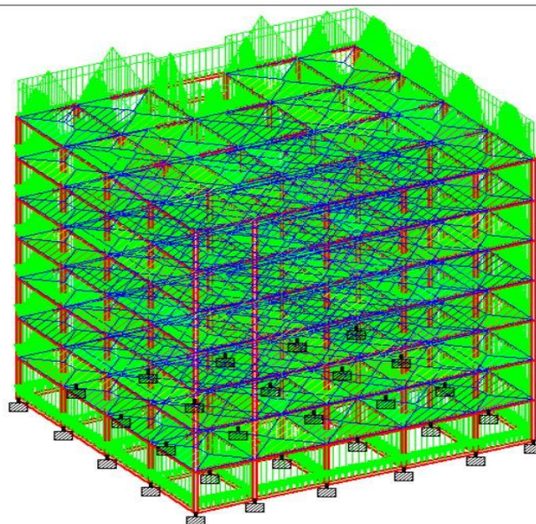
Fig5:Dead Load of g+7building
