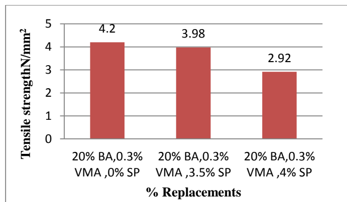
Fig. 3.4 Comparison of tensile strength at 28 days curing
