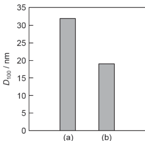
Figure 5. The D_{100} values of hydroxyapatite (HAP) prepared from, (a) CALPHOS and (b) Suc-20, calculated by using of Scherrer equation [ D_{100} = K\lambda / (\beta \cos\theta) ] .
