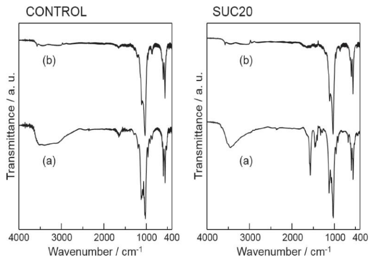
Figure 4. The FTIR spectra of samples CONTROL and SUC20 under {before (a), and after (b)} hydrothermal treatment at 180 °C for 3 hour.
