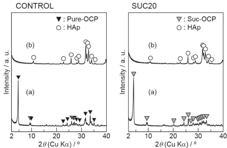
Figure 3. The XRD patterns of samples CONTROL and SUC20 under {before (a), and after (b)} hydrothermal treatment at 180 °C for 3 hour.
