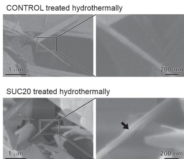
Figure 2. SEM magnification images of samples CONTROL or CALPHOS and SUC-20 (T.Yokoi et al) under by hydrothermally treatment at 180°C for 3hr, where the black arrow indicates a dark line at center of HAP nanocrystal system.
