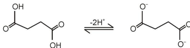
Figure 1. The structure of succinic acid ( \text{HOOC} \cdot (\text{CH}_2)_2 \cdot \text{COOH} ) and its succinate ion ( \text{OOC} \cdot (\text{CH}_2)_2 \cdot \text{COO}^{2-} ).
