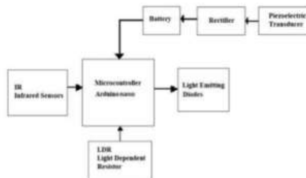
Figure1. Block Diagram
