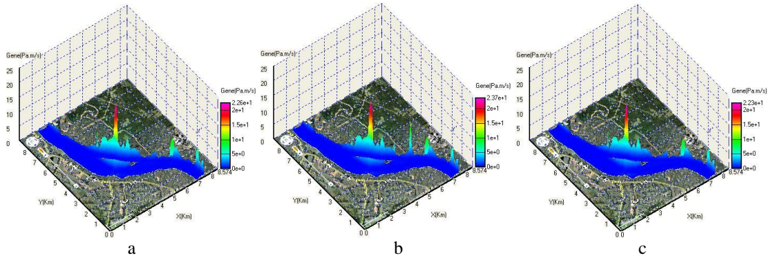
Fig. 10 P_k distributions, calculated by \tilde{k} - \tilde{\omega} , \tilde{k} - \tilde{\epsilon} and \tilde{k} - \tilde{w} models
