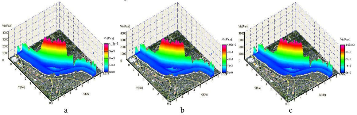
Fig. 9 3D \tilde{\mu}_{eff} distributions, calculated by \tilde{k} - \tilde{\omega} , \tilde{k} - \tilde{\epsilon} and \tilde{k} - \tilde{w} models.
