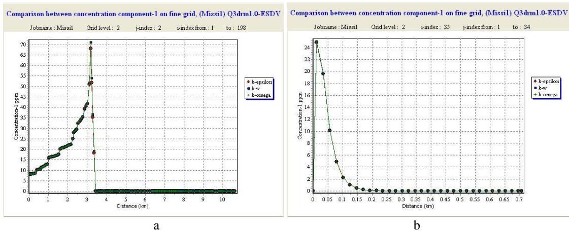
Fig. 11 Concentrations at a: i from 1 to 198 and j=2 ; b: i=35 and j from 1 to 34.
