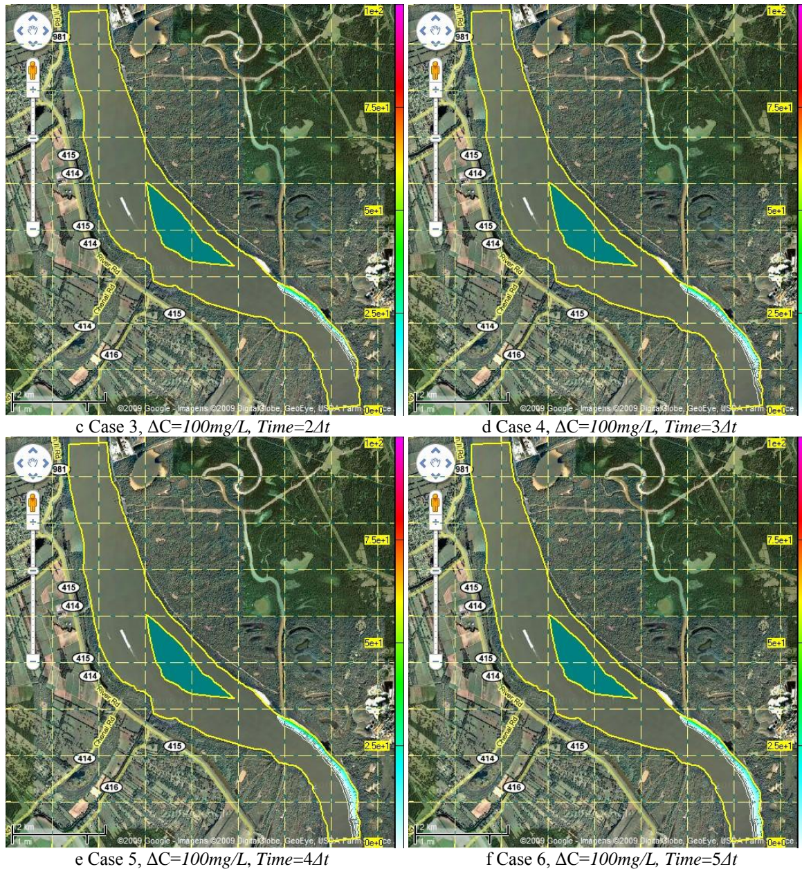
Fig. 13 Contaminant plume development.
