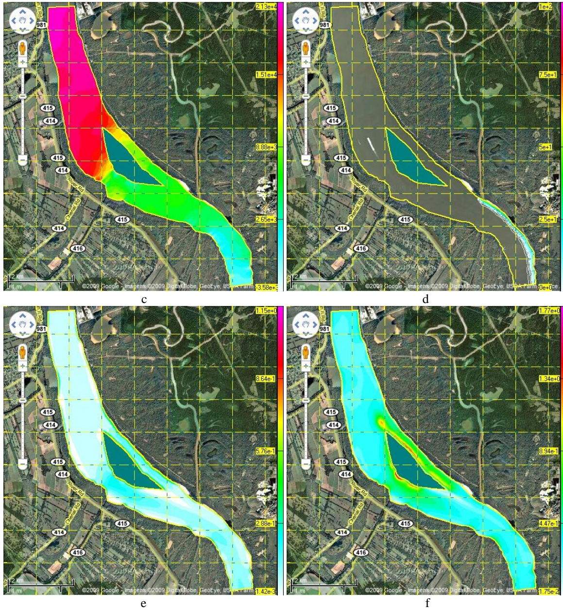
Fig. 6 A part of results, calculated by \tilde{k} - \tilde{\omega} model.
