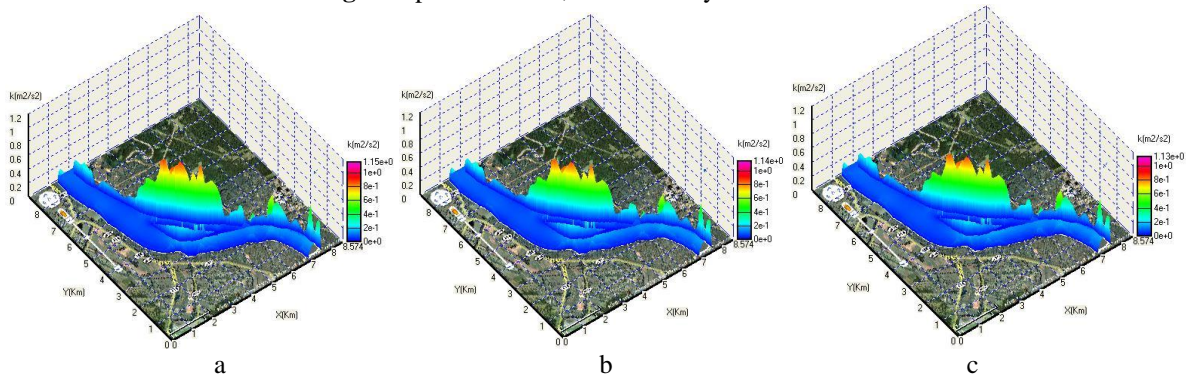
Fig. 7 3D \tilde{k} distributions, calculated by \tilde{k} - \tilde{\omega} , \tilde{k} - \tilde{\varepsilon} and \tilde{k} - \tilde{\omega} models.
