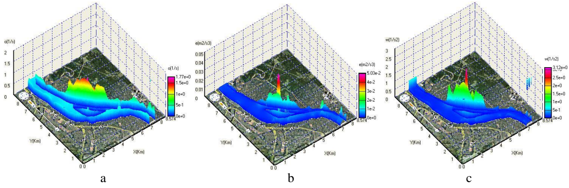
Fig. 8 3D \tilde{\omega} , \tilde{\epsilon} and \tilde{w} distributions.
