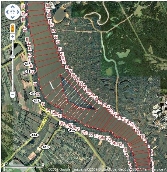
Fig. 2 Map, plotted by interface .
