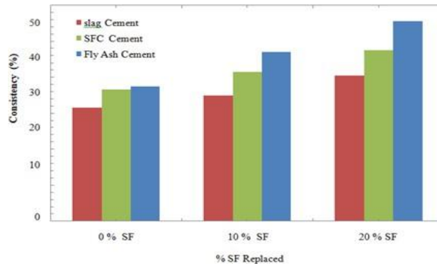
Fig-1 Consistency of Mortar
