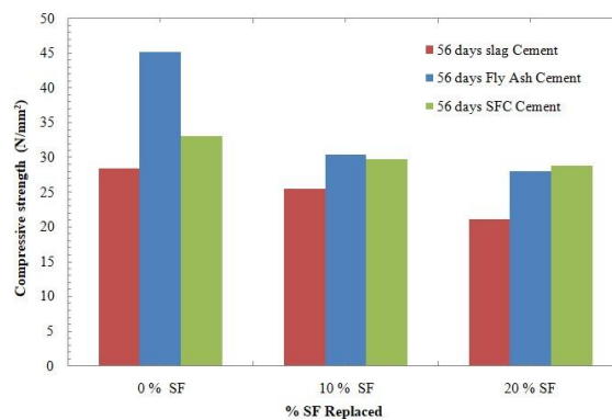
Fig-7: Compressive strength of concrete for 56 days
