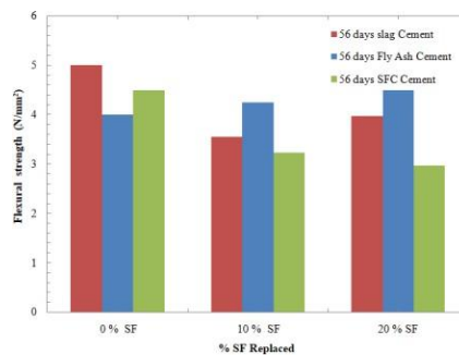
Fig-8: Flexural strength of concrete for 56 days
