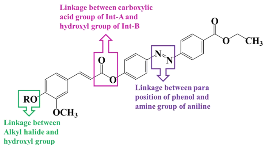
Figure 8. Structure of Series-D.
