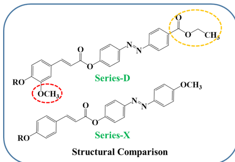
Figure 13. Structural comparison of Series-D and X.
