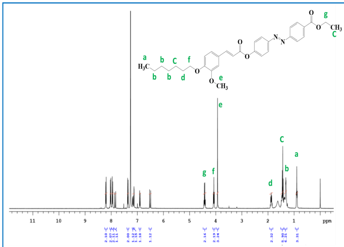
Figure 3. ^1\text{H} -NMR spectra of D-7 compound.
