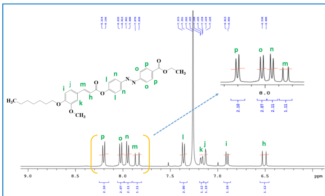
Figure 4. ^1\text{H} -NMR Aromatic region of D-7 compound.
