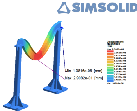
Figure 7A. Results of displacement on Simcenter 3D software.
