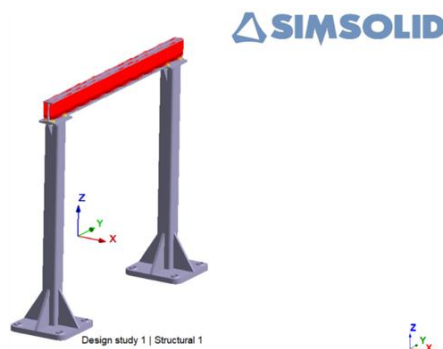
Figure 6. Set boundary conditions and apply forces.
