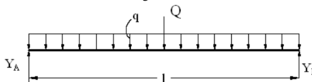
Figure 1. Load diagram acting on the main beam
