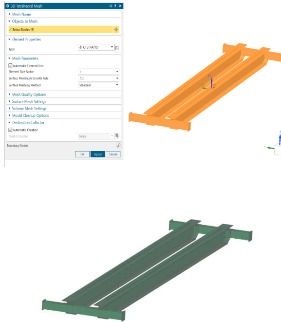
Figure 8. Automatic mesh generation by softwar
