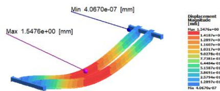
Figure 10B. Stress and displacement results using Simsolid software
