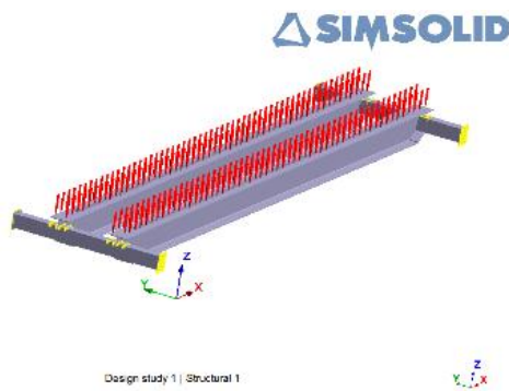
Figure 9. Set boundary conditions and apply forces.
