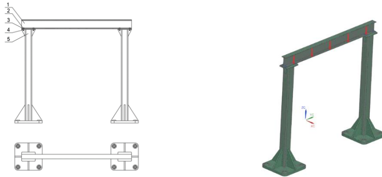
Figure 3. Beam 1
