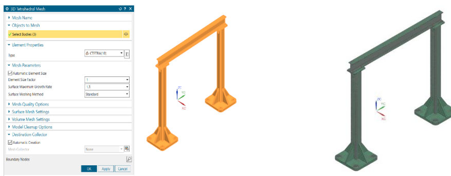
Figure 5. Automatic mesh generation by software
