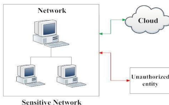
Figure2:illegalaccessesof dataCloud
