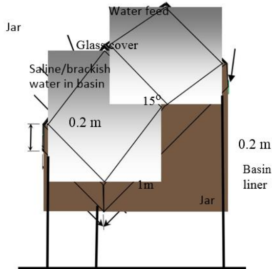
double slope passive solar still
