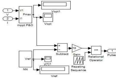
Fig.8. MATLAB/SIMULINK arrangement of entire PV system.
