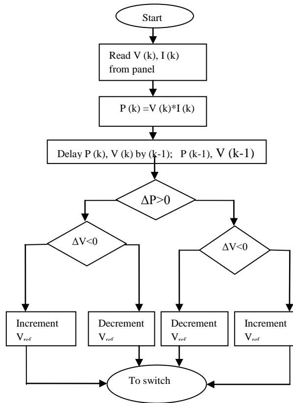
Fig.3. Flow chart of P&O Algorithm.
