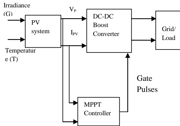
Fig. 1. Block diagram of a PV system.
