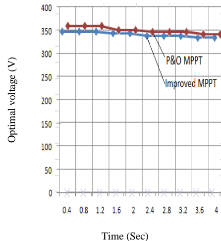
Fig.12. Comparison of conventional and improved MPPT Techniques (a) Maximum power comparison (b) Optimal voltage comparison
