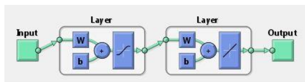
Fig.5. Back-propagation neural network for MPPT.
