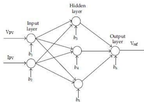
Fig.4. Architecture of Back-propagation neural network.
