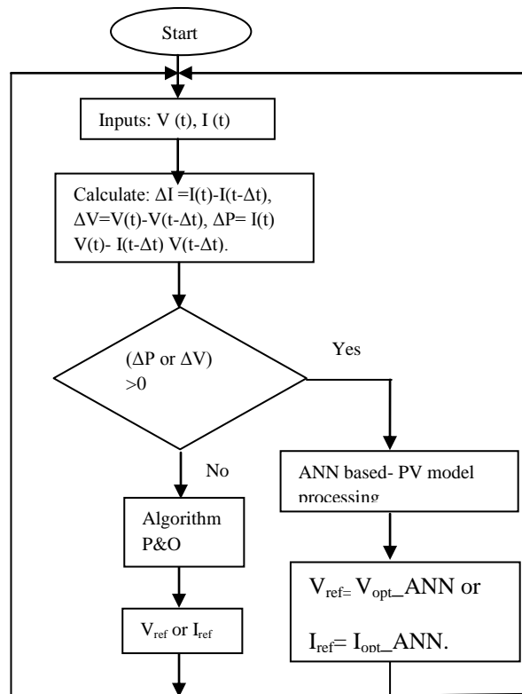
Fig.6. Flow chart of proposed ANN based Algorithm.
