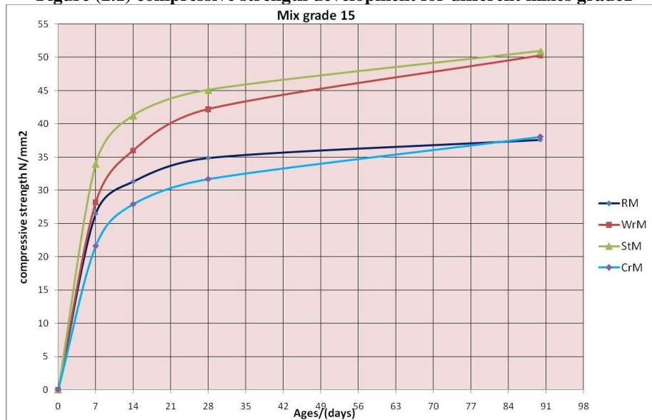
Figure (2.1) compressive strength development for different mixes grade 1
