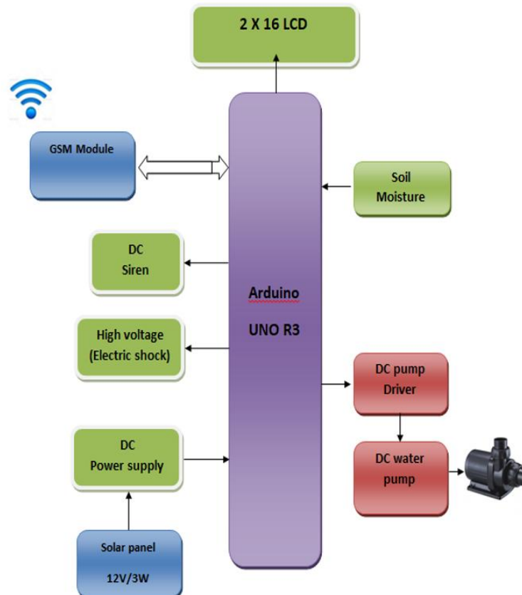
Fig (1): -Solar based automatic irrigation system
