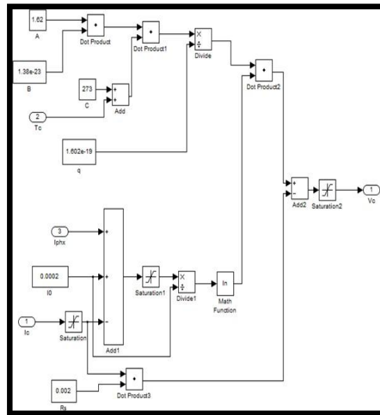
Fig.3: Simulink model of Vc
