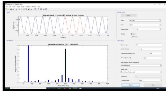
Fig. 10: Power Factor of Three Phase Source with Buck Converter.
