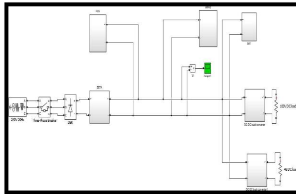
Fig.7: Simulink Modelling of Proposed Test System
