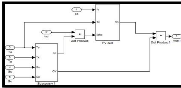
Fig.5: Combined diagram of CV, CI & Vc Mathematical Models.
