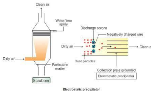
Fig. 7. Electrostatic Precipitator
