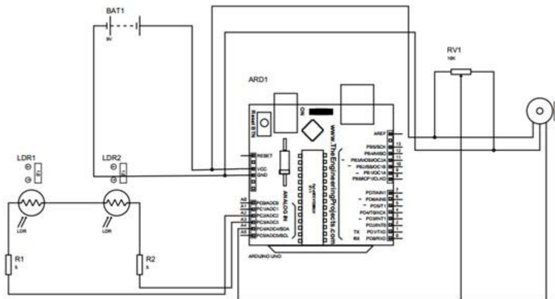
Figure 3: Schematic diagram of the solar panel tracking system.
