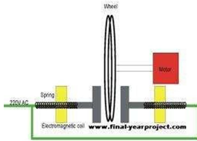
Fig 1.1 Schematic Diagram of Principle of Electromagnetic Braking System
