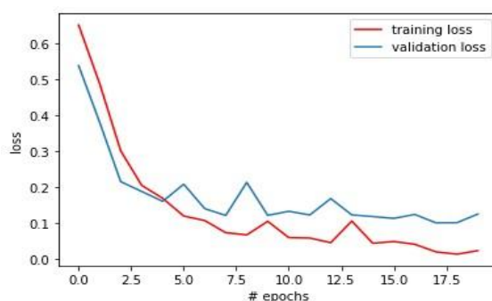
Fig. 6. # epochs vs loss corresponding to dataset 1
