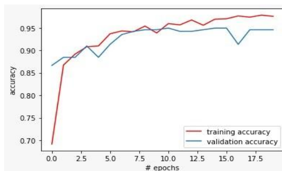
Fig. 9. # epochs vs accuracy corresponding to dataset 2
