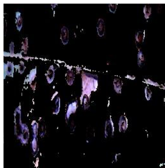
Figure 8. Segmented Image
