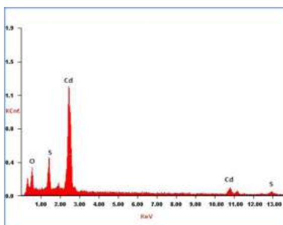
Fig. 2. EDAX spectrum of CdS thin film of thickness 930 Å
