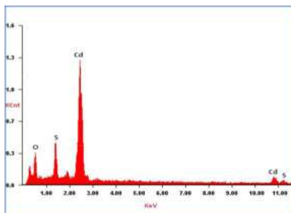
Fig. 3. EDAX spectrum of CdS thin film of thickness 2550 Å
