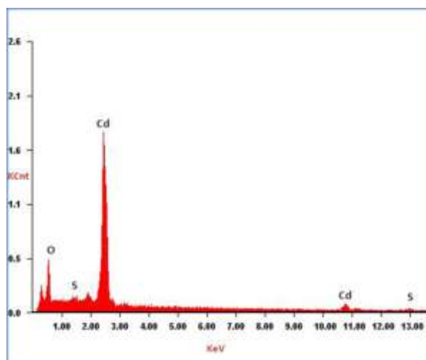
Fig. 1. EDAX spectrum of CdS thin film of thickness 880 Å
