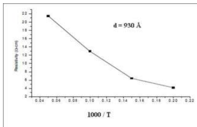
Fig. 5. Resistivity Vs ( 1000/T ) of CdS thin film of thickness 930 Å.
