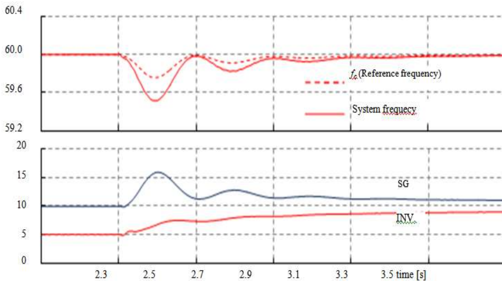
Figure 5. Frequency and active powers after a load variation when k_c = 0.5 .
