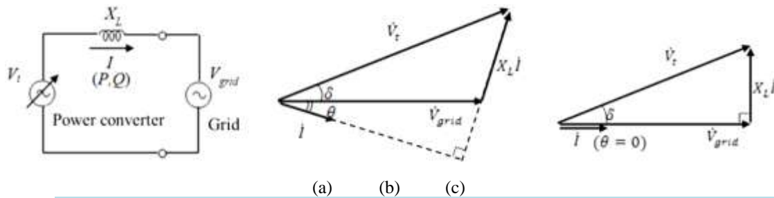
Figure 3. Reactive power regulation of the converter. (a) A simplified equivalent circuit, (b) Phase-shifted output voltage phasors, (c) Regulated output voltage phasor.
