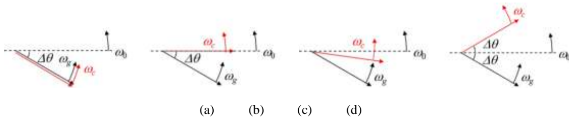
Figure 2. Various placements of the converter output voltage phasors. (a) k_c = 0.0 , (b) k_c = 1.0 , (c) 0.0 < k_c < 1.0 , (d) k_c = 2.0 .
