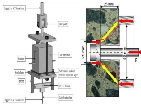
Fig. 4 and Fig. 5. Schematic of Pullout test apparatus
